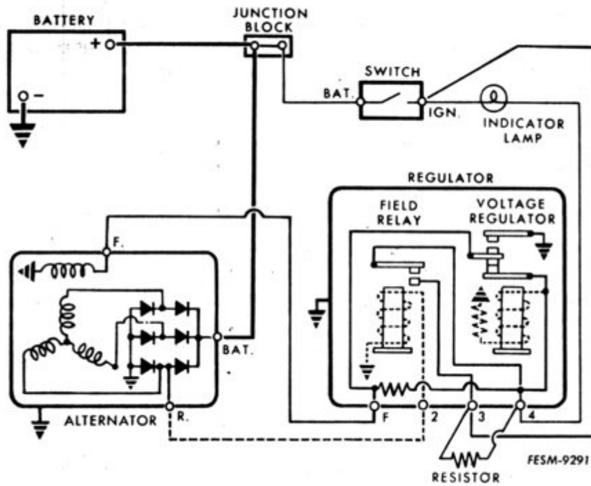
Fig. 1 - Alternator with external voltage regulator.
