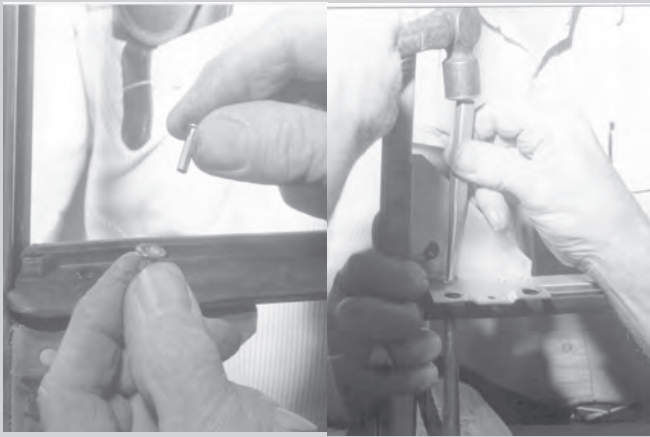
Insert new rivets within original sleeves.
