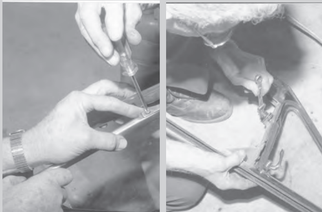
On bench, remove screws in hinge of vent window. With a wrench, remove the nut on the anchoring post of the window to release springs.
