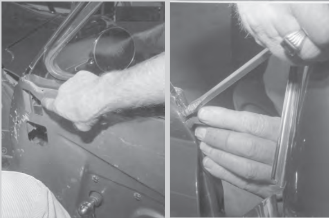
Remove bolt and screw at front of door.
